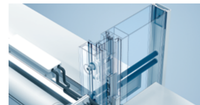
cabling between integration profile and post
