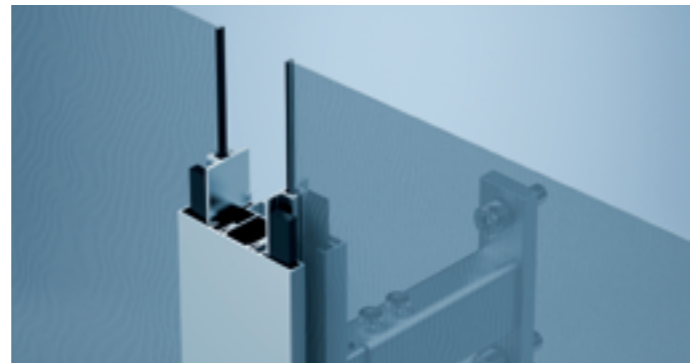
centre guide rail heroal GR 37
